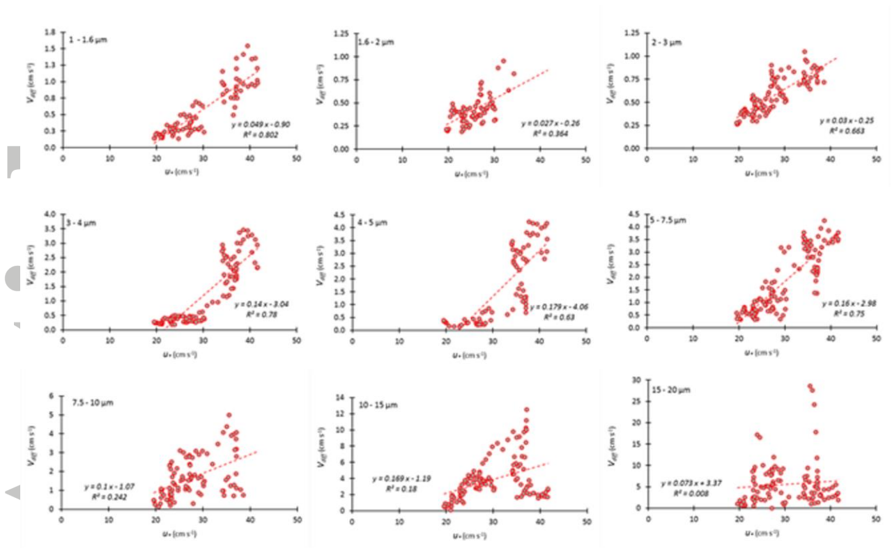
Figure 15. V_{diff} versus u_* for different size classes on 18 June 2006 (only V_{diff} for which the difference between C_{6.5} - C_{2.1} is > 5\% are reported, Table S1 in Supporting Information provided the number of data used for each channel).
