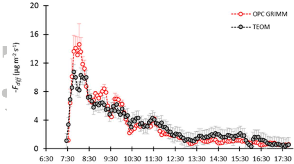
Figure 11. Time evolution of the diffusive dry deposition flux of dust on 18 June 2006. The vertical bars correspond to the standard deviation of (C_{6.5m} - C_{2.1m}) over the 20-minute averaging period. Gray points: TEOM ® ; red points: OPC.
