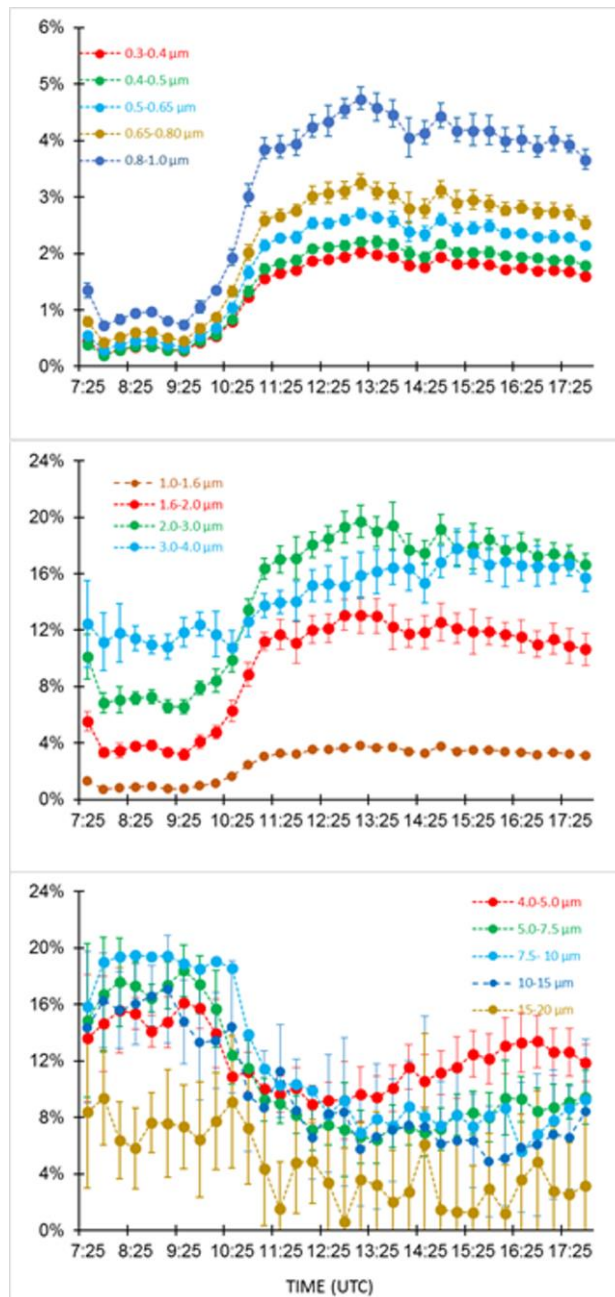
Figure 7. Temporal evolution of the mass-size distributions of particles for the various size classes of the optical particle counter at 2.1 m for 18 June 2006. The data are averaging over 20-minute periods and the vertical bars represent the standard deviation of the data for each 20-minute period.
