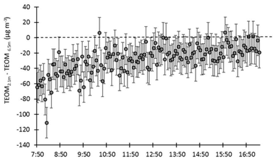
Figure 5. Differences between the 20-minute averaged particulate matter concentrations (with a slipping time step of 4 minutes) measured by the TEOM ® instruments at two different heights (2.1 and 6.5 m) on 18 June 2006.
