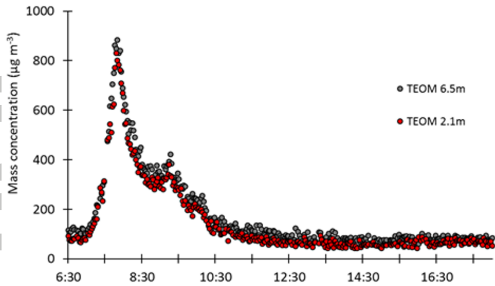
Figure 4. Evolution of the particulate matter mass concentrations measured by the TEOM ® instruments on 18 June 2006.
