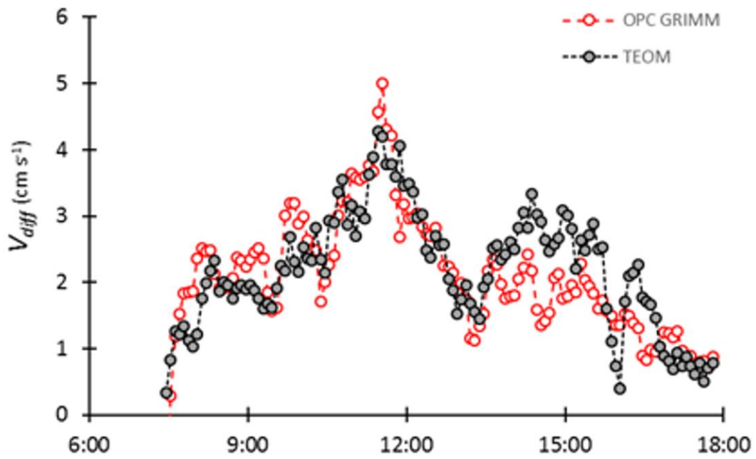
Figure 13. Diffusive dry deposition velocities derived from the TEOM ® s (gray points) and OPCs (red points) measurements for the 18 June 0727-1747 UTC period.
