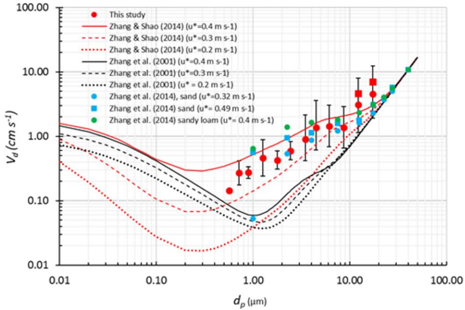
Figure 17. Comparison between measured dry deposition velocities (red points) and the Zhang et al. (2001) (black lines) and Zhang and Shao (2014) (red lines) dry deposition schemes for three different wind friction velocities (0.2, 0.3 and 0.4 m s -1 ). For particles larger than 10 μm in diameter, red circles correspond to the 0737-1002 UTC period and the red squares to the period 1007-1757 UTC. Only V_d for which the difference between C_{6.5} - C_{2.1} is > 5% are accounted for. Dry deposition velocities measured in a wind tunnel over sand (blue points) and sandy loam (green points) surfaces by Zhang et al. (2014) are also reported.
