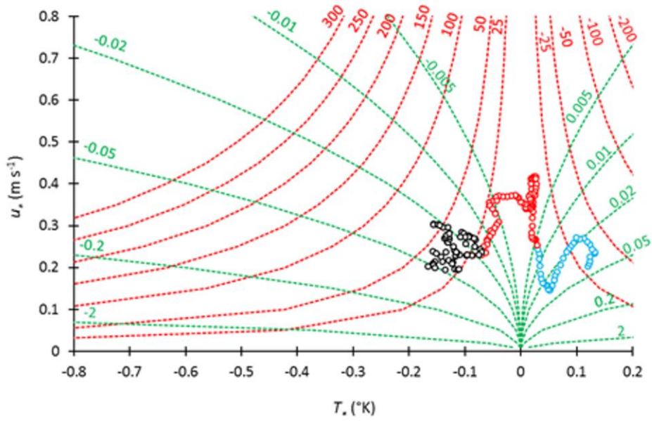
Figure 10. Localization of consecutive 5-minute periods for 18 June 2006 in a diagram u_* = f(T_*) . Blue points: 0402 to 0657 UTC; red points: 0702 to 1307 UTC; black points: 1312 to 1757 UTC. The green lines correspond to isolines of 1/L ( \text{m}^{-1} ) and red ones to isolines of the sensible heat flux, H_s ( \text{W m}^{-2} ).
