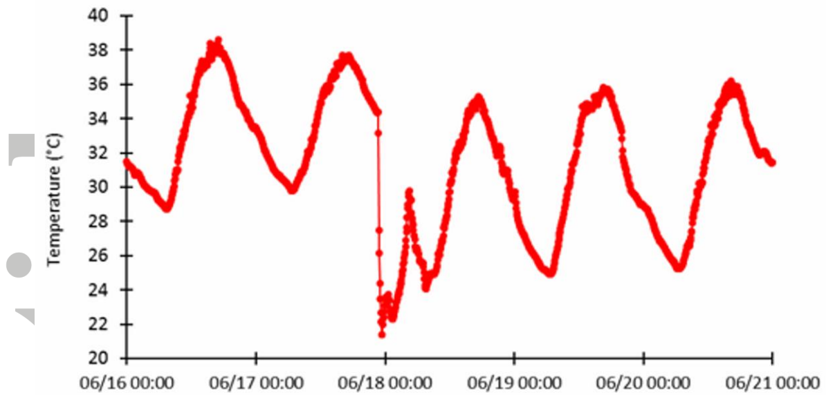
Figure 9. Time series of temperature at 6.5 m at Banizoumbou (Niger) for the 15-21 June 2006 period. The abrupt change in temperature occurring on 17 June 2200 UTC is due to the arrival of the mesoscale convective system also responsible for the dust emission.
