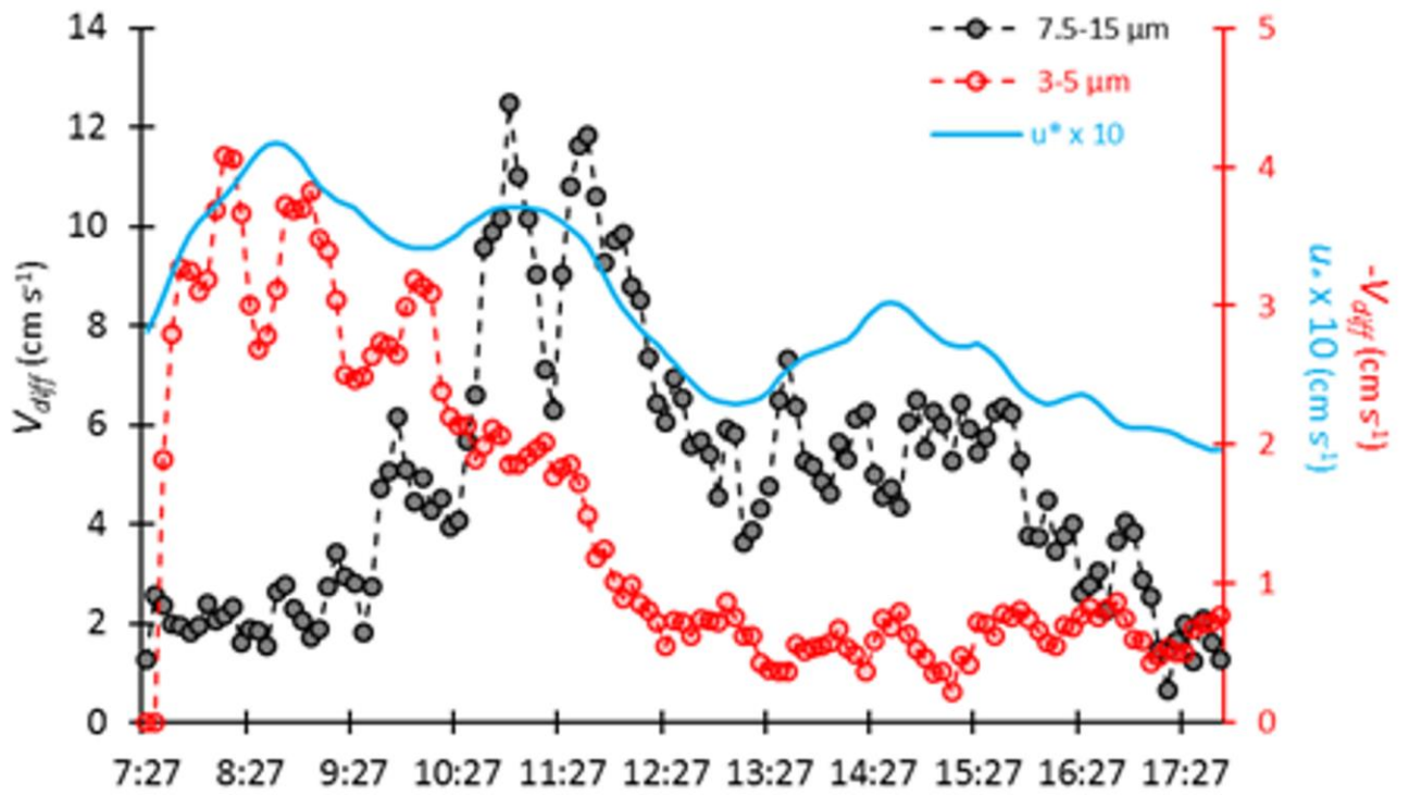
Figure 14. Diffusive dry deposition velocity of particles for the 3-5 \mu\text{m} (red points) and 7.5-15 \mu\text{m} (gray points) particle size ranges and wind friction velocity (blue line) during 18 June 2006.
