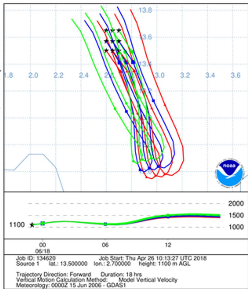
Figure 3. 18 hours forward trajectories starting on 17 June 2006 2300 UTC from an area ranging from 13.5° N-13.65° N and 2.6° E-2.7° E (black stars).
