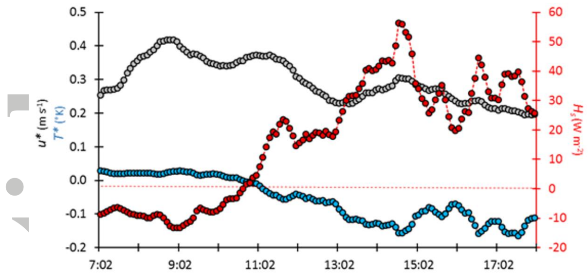
Figure 8. Temporal evolution of the wind friction velocity ( \text{m s}^{-1} ), the temperature scale (K) and the sensible heat flux ( \text{W m}^{-2} ) on 18 June 2006.
